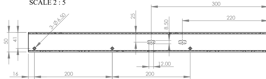
DETAIL D SCALE 2 : 5
