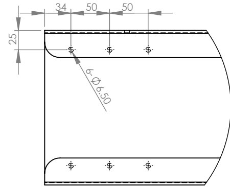
DETAIL E SCALE 1 : 5
